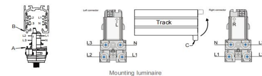
Mounting luminaire
